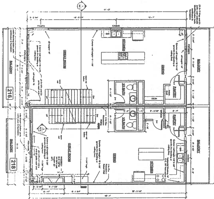
① Second Floor 1/16" = 1'-0"
