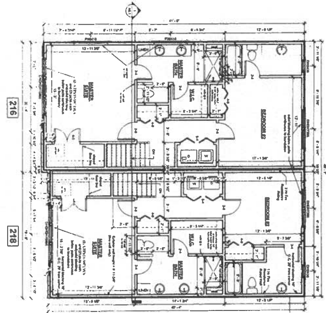
② Third Floor 1/16" = 1'-0"
